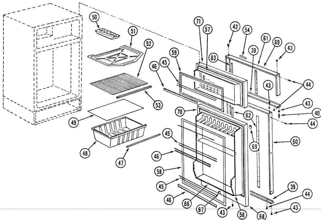
Figure 37-1. Refrigerator
