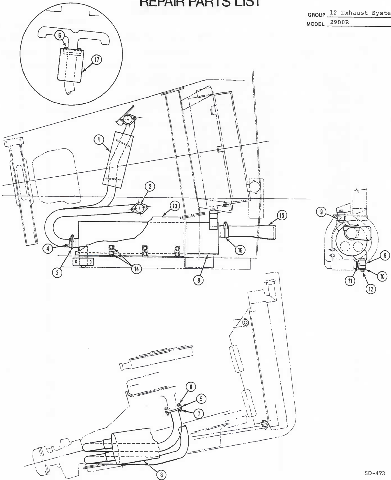
Figure 12-1. Exhaust System
