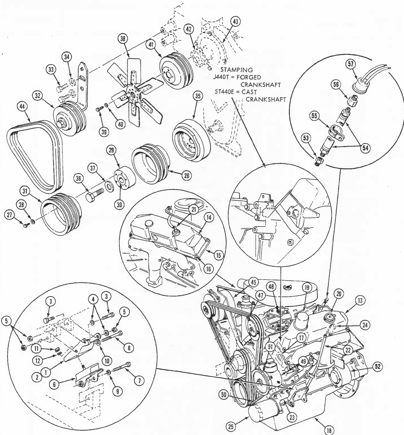
Figure 15-1. Engine Assembly
