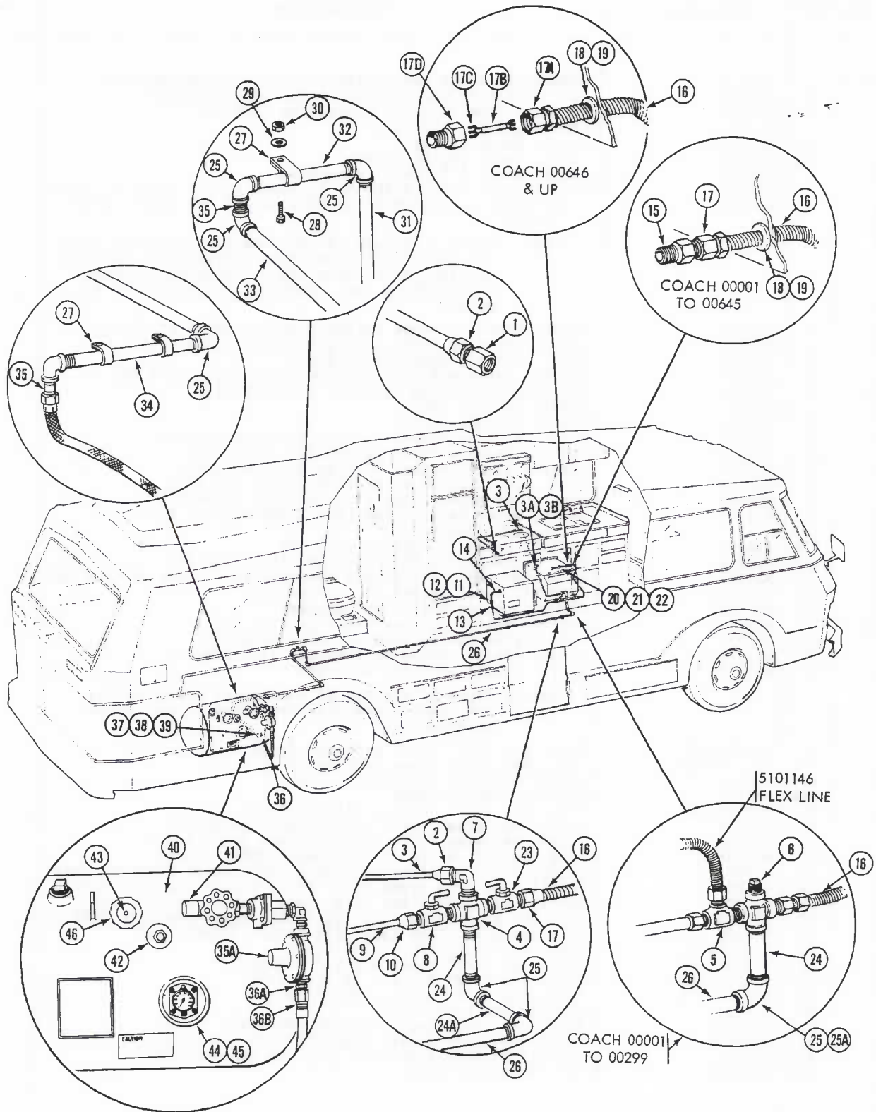
Figure 38-1. LPG System
